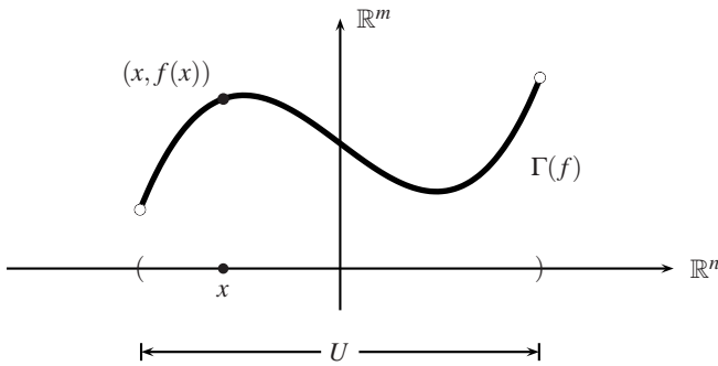
Fig. 5.6. The graph of a smooth function f: \mathbb{R}^n \supset U \rightarrow \mathbb{R}^m .
